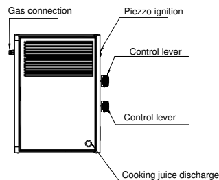
Description of the Plancha (top view)
